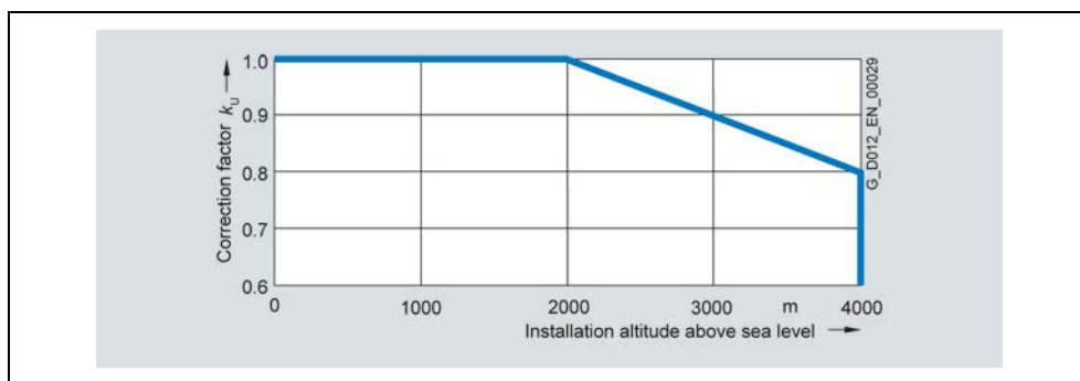
Fig. 4-9 Derating factor k_u
