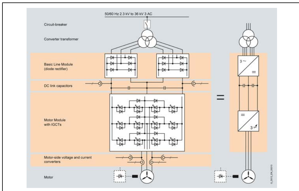
Fig. 3-3 Block diagram
