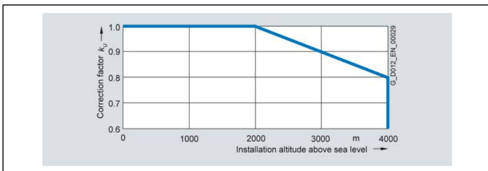
Fig. 2-13 Derating factor k_U
