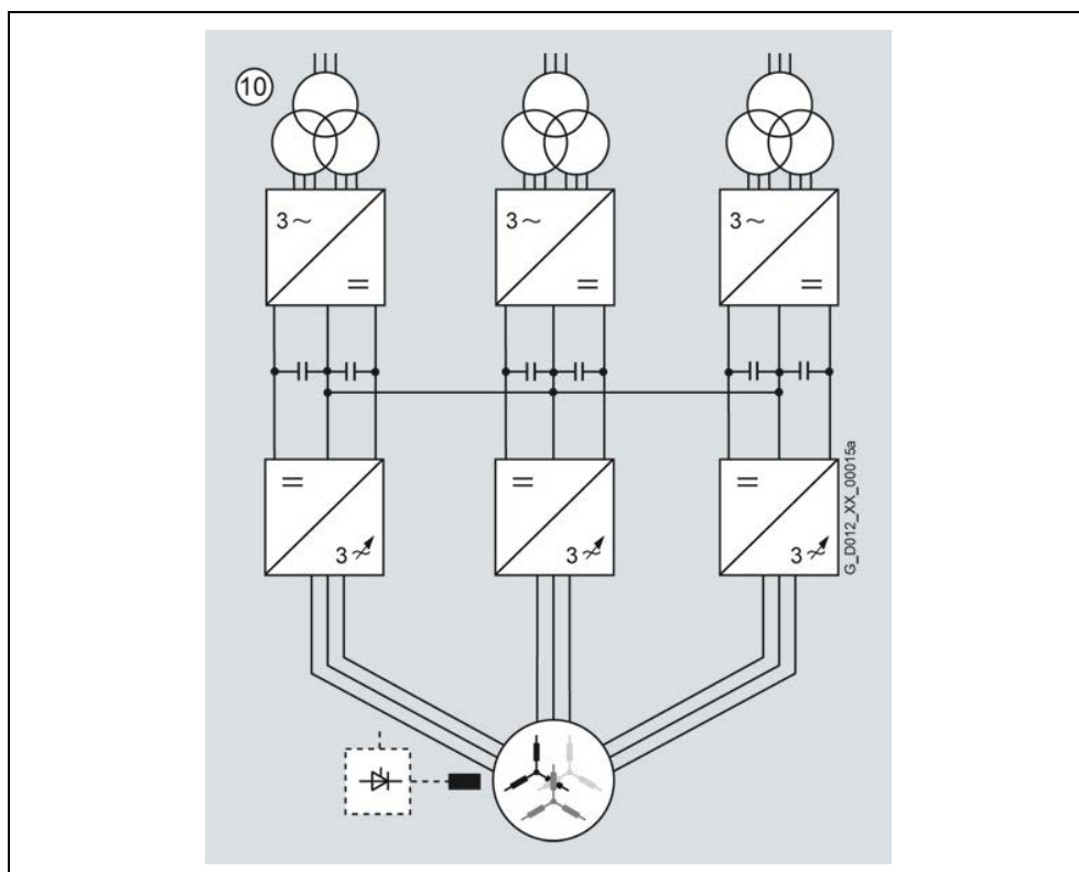
Fig. 3-8 Increased power rating by connecting three converter units in parallel 1) , 36-pulse infeed
