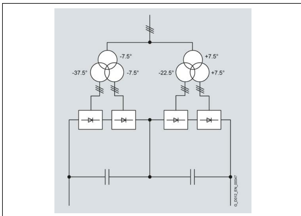
Fig. 7-8 SINAMICS GM150 in the IGCT version, 24-pulse infeed by connecting two Basic Line Modules in series (absolute values of the individual phase offset angles are examples only)
