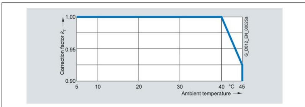
Fig. 2-11 Derating factor k_T (ambient temperature)
