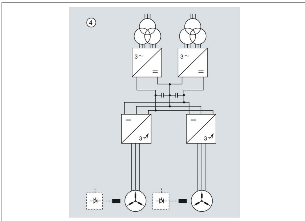
Fig. 2-7 DC bus configuration with two motors connected to a common DC link
