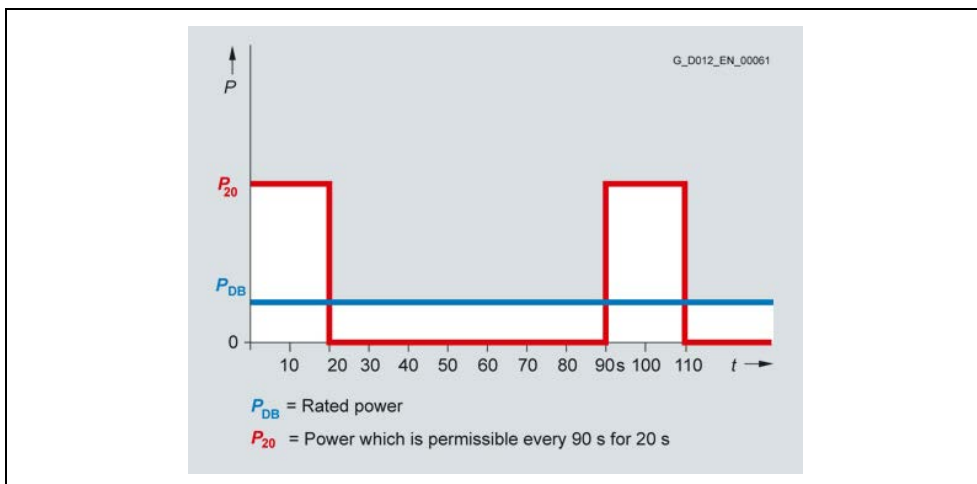
Fig. 7-6 Load diagram
