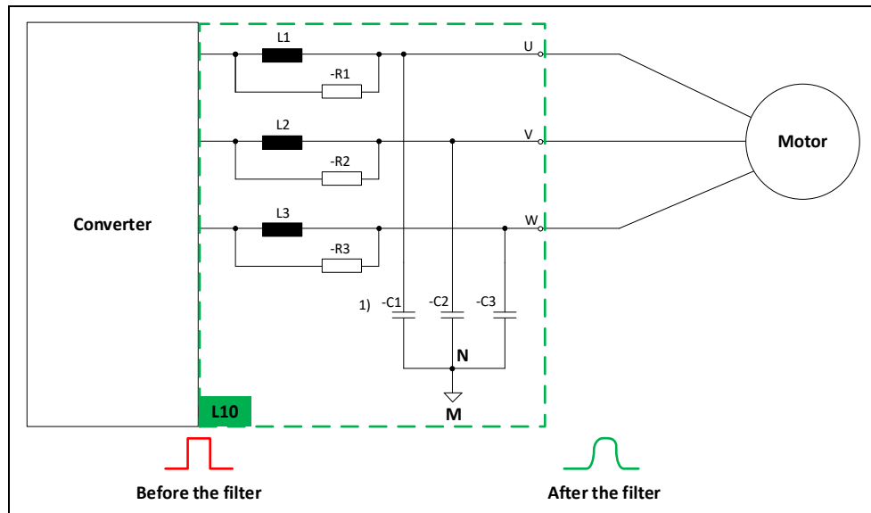
Fig. 7-2 Block diagram for Option L10 (N: Filter neutral point; M: Converter mid-point)
