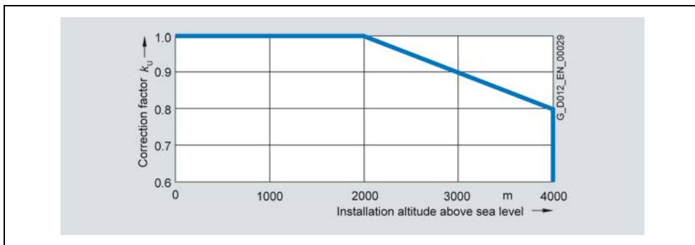
Fig. 5-12 Derating factor k_u
