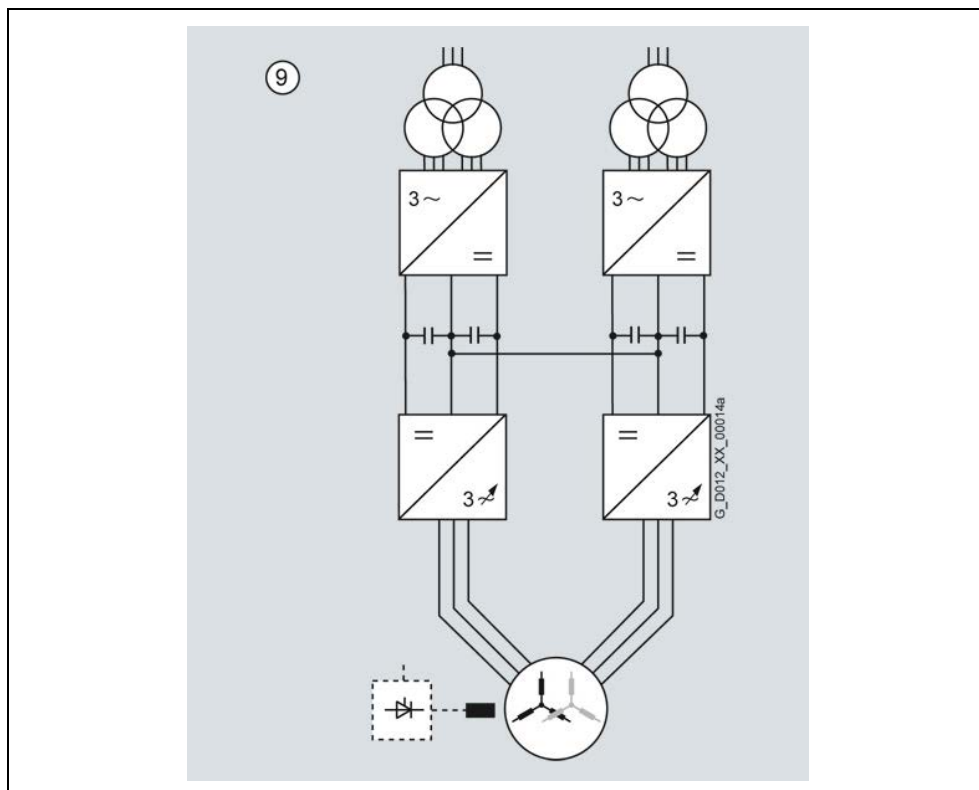
Fig. 3-7 Increased power rating by connecting two converter units in parallel 1) , 24-pulse infeed
