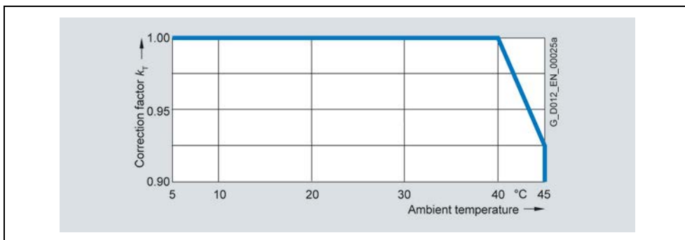
Fig. 4-7 Derating factor k_T (ambient temperature)
