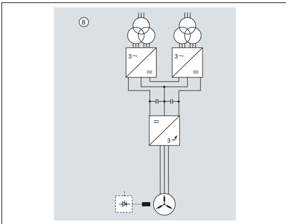
Fig. 3-6 24-pulse infeed by connecting two Basic Line Modules in series: Option N15
