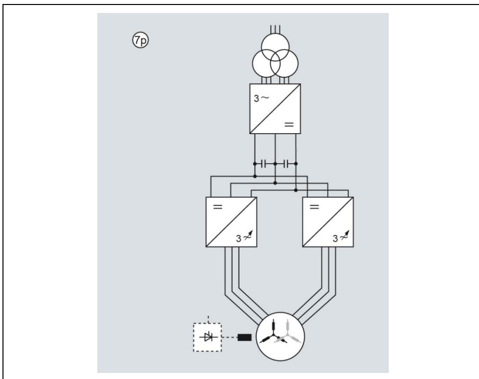
Fig. 3-5 Parallel circuit, 12-pulse infeed
