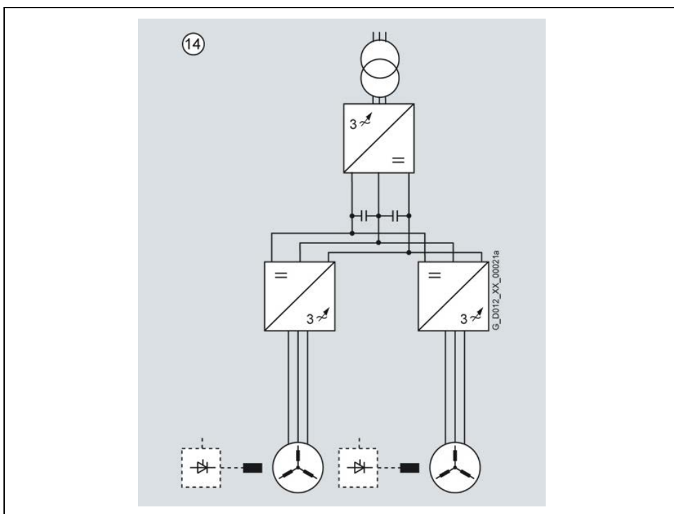
Fig. 5-7 DC bus configuration with two motors connected to a common DC link
