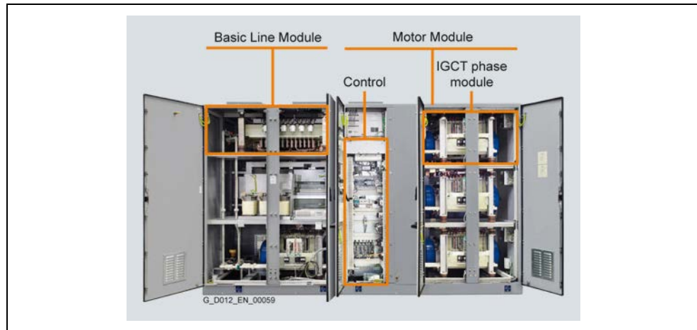
Fig. 6-1 SINAMICS SM150 in the IGCT version with diode infeed (principle design without cooling unit)
