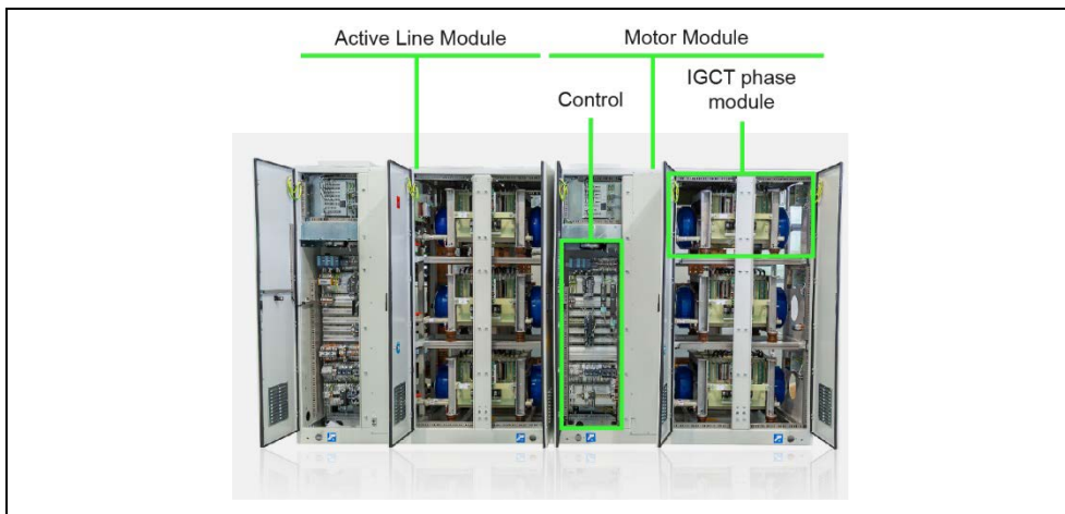
Fig. 5-2 SINAMICS SM150 in the IGCT version, internal design (without cooling unit)
