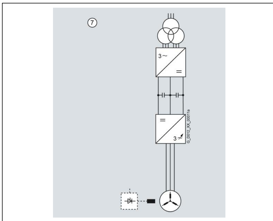
Fig. 3-4 Basic circuit, 12-pulse infeed
