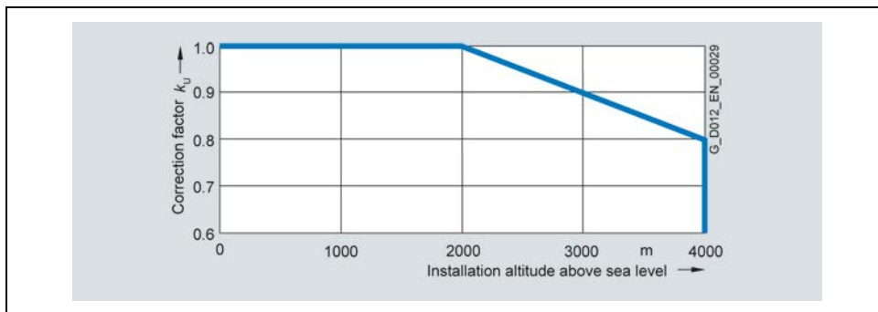
Fig. 3-12 Derating factor k_U
