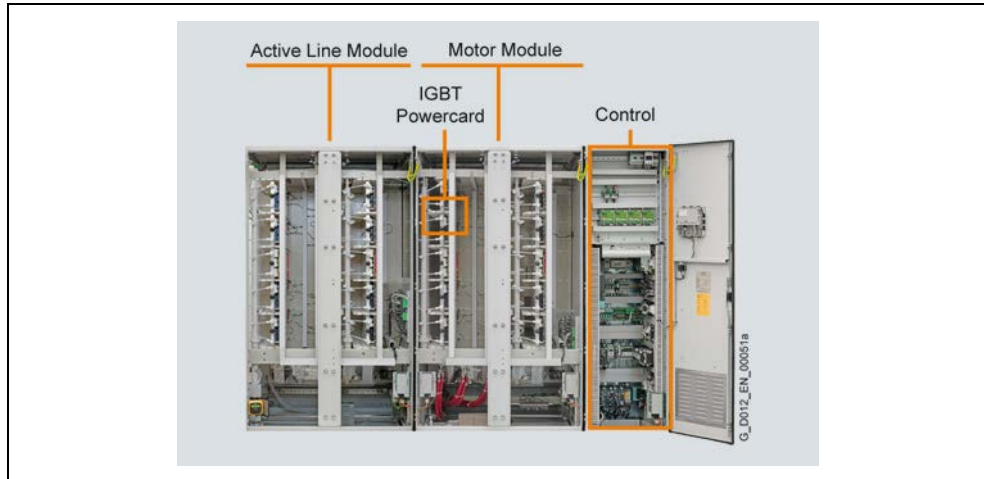
Fig. 4-2 SINAMICS SM150 in the IGBT version, water cooling, internal design without cooling unit
