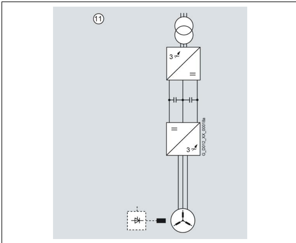
Fig. 4-4 Basic circuit
