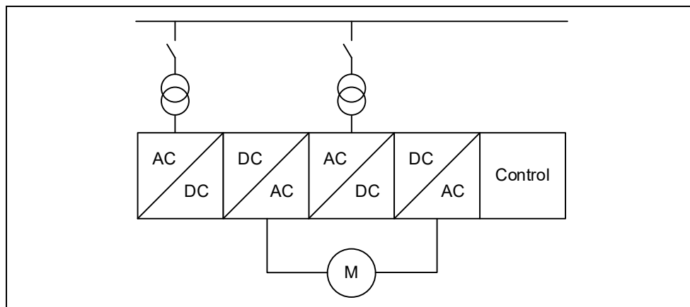
Fig. 7-4 Option L38: Redundant power section for parallel circuit configuration
