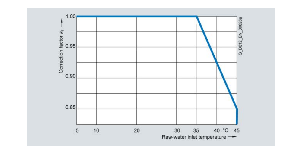
Fig. 3-11 Derating factor k_T (raw water intake temperature)
