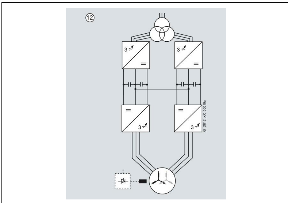
Fig. 5-5 Power rating increased by connecting two converter units in parallel (additional reduction of the line harmonics) 1)
