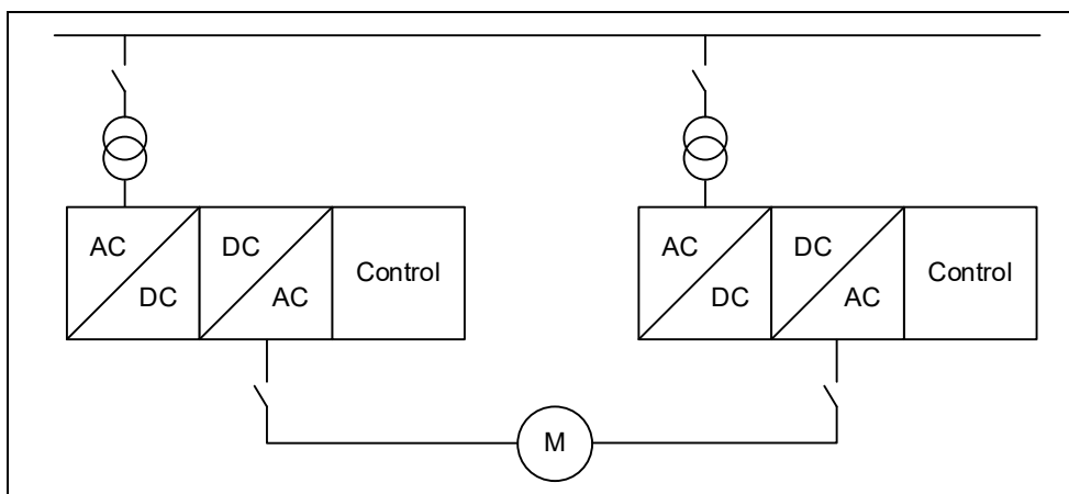
Fig. 7-3 Option L35: Redundant power section and control
