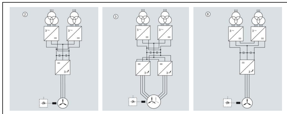
(2) SINAMICS GM150 in the IGBT version, basic circuit 2.3 kV to 4.16 kV (option N15)
