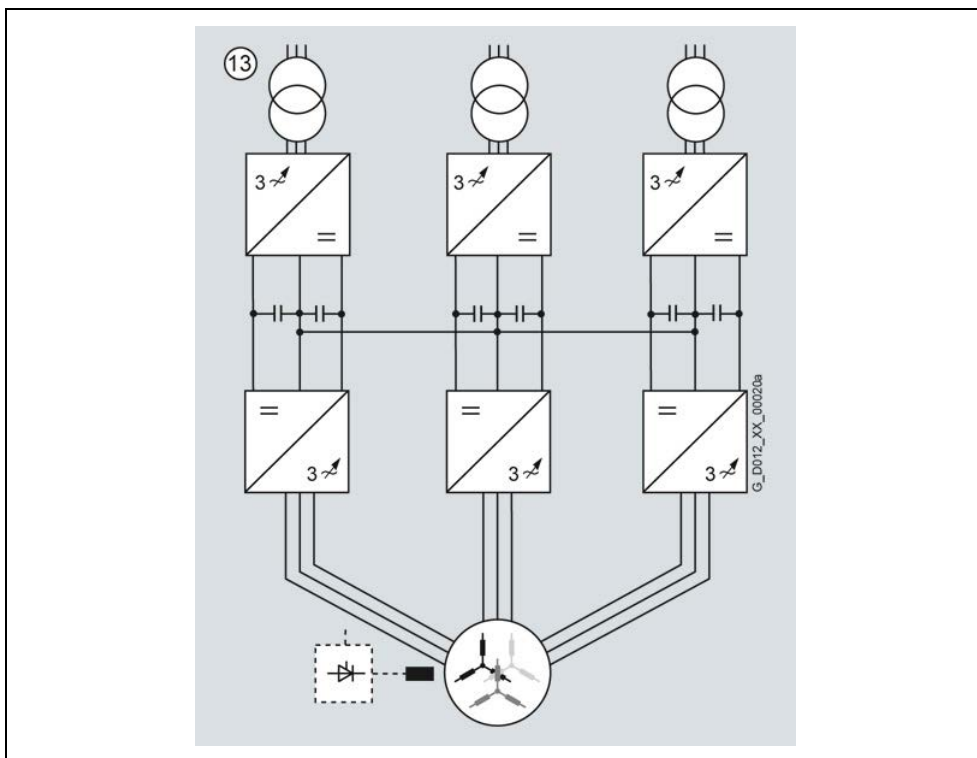
Fig. 5-6 Power rating increased by connecting three converter units in parallel (additional reduction of the line harmonics) 1)
