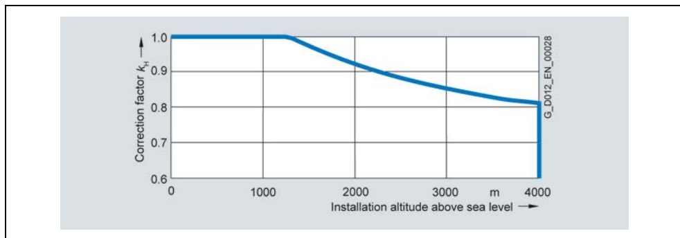
Fig. 5-10 Derating factor k_H for water cooling
