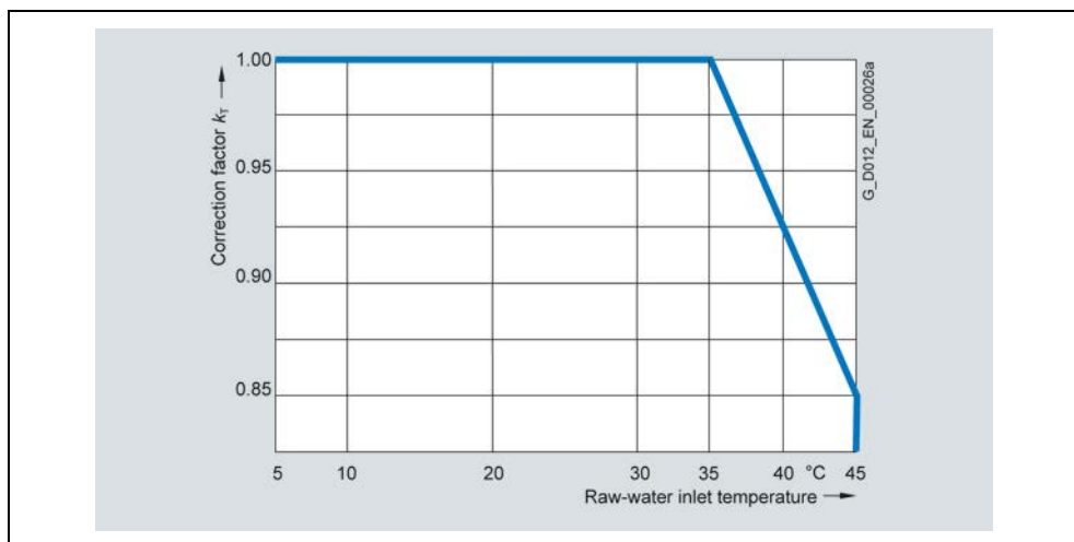
Fig. 5-11 Derating factor k_T (raw water intake temperature)
