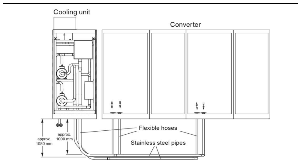
Fig. 11-1 Piping for SINAMICS GM150 in the IGCT version and for SINAMICS SM150 in the IGCT version
