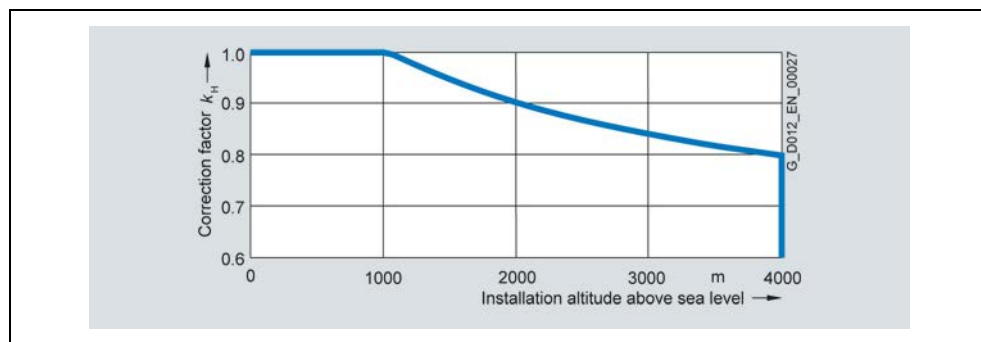
Fig. 4-5 Derating factor k_H for air cooling
