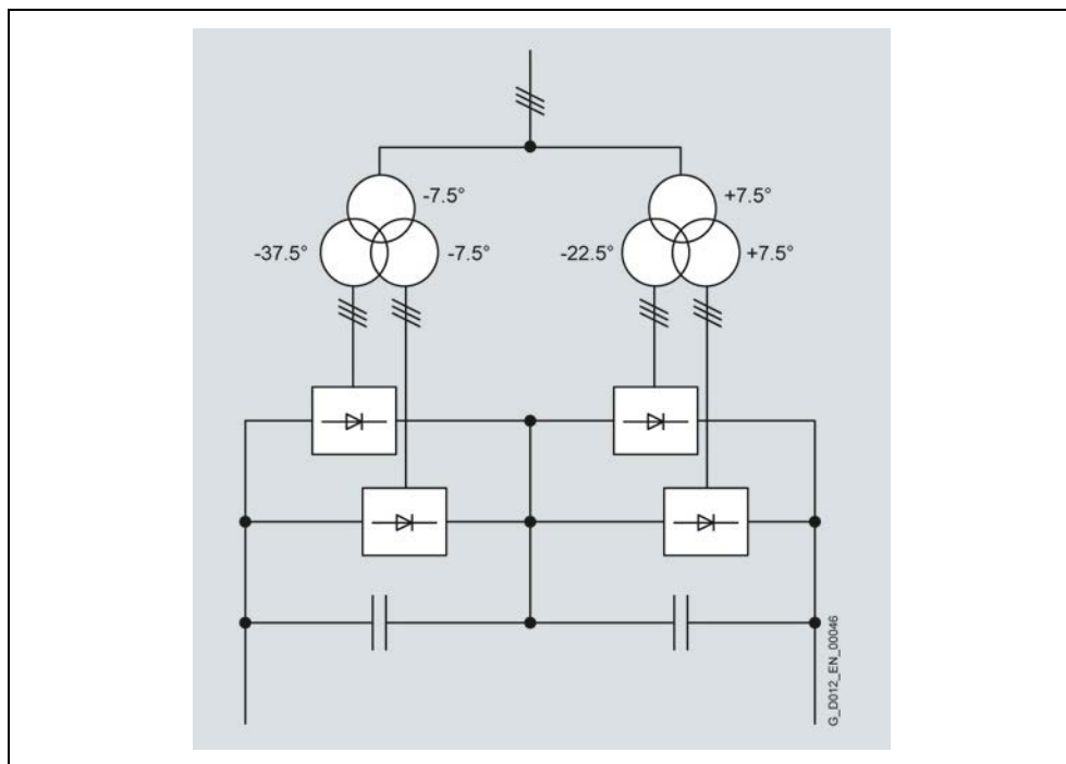
Fig. 7-7 SINAMICS GM150 in the IGBT version, 24-pulse infeed by connecting two Basic Line Modules in parallel (absolute values of the individual phase shift angles as example only)
