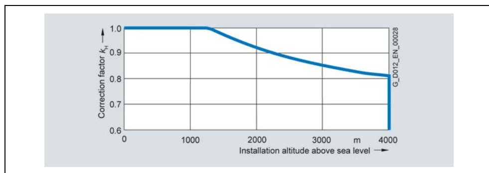
Fig. 3-10 Derating factor k_H for water cooling
