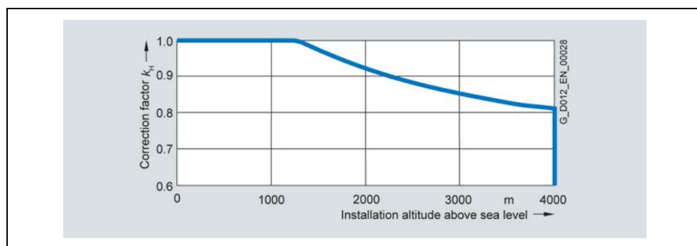
Fig. 4-6 Derating factor k_H for water cooling
