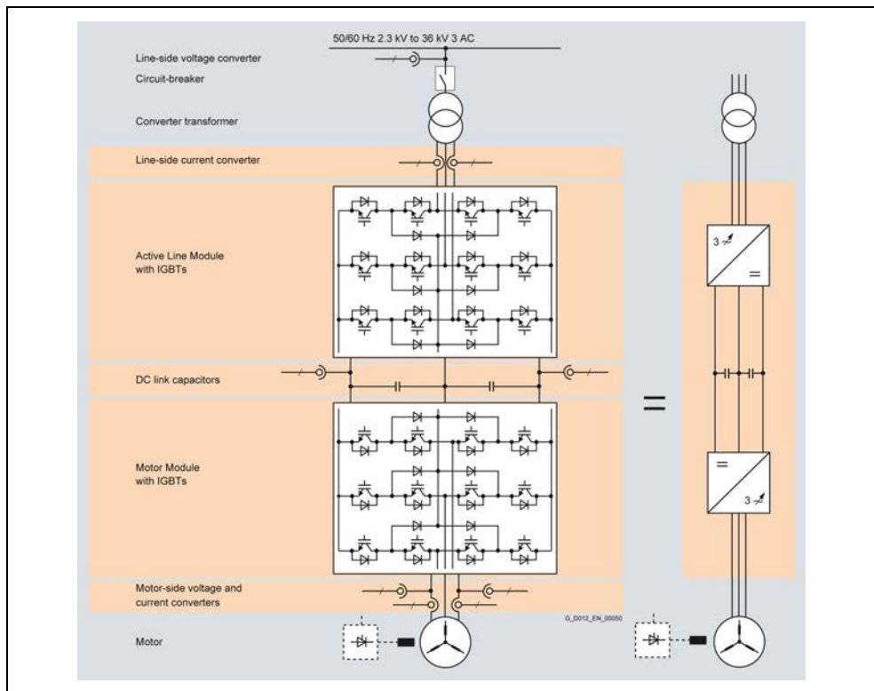
Fig. 4-3 Block diagram
