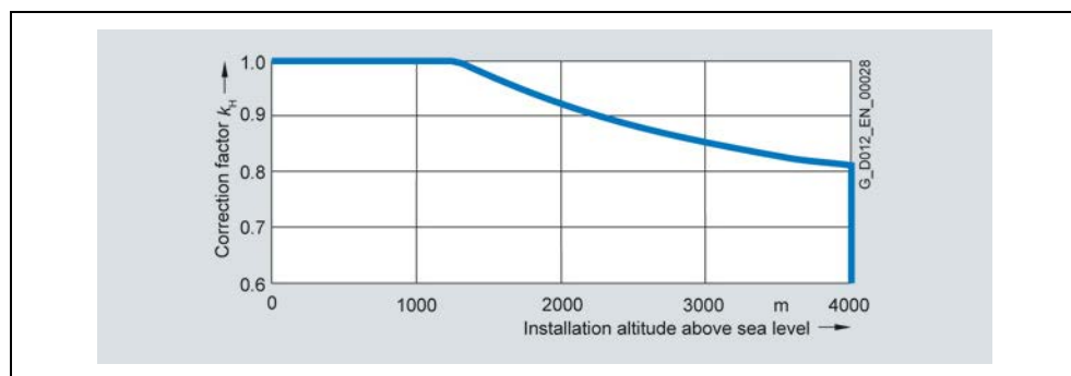
Fig. 2-10 Derating factor k_H for water cooling
