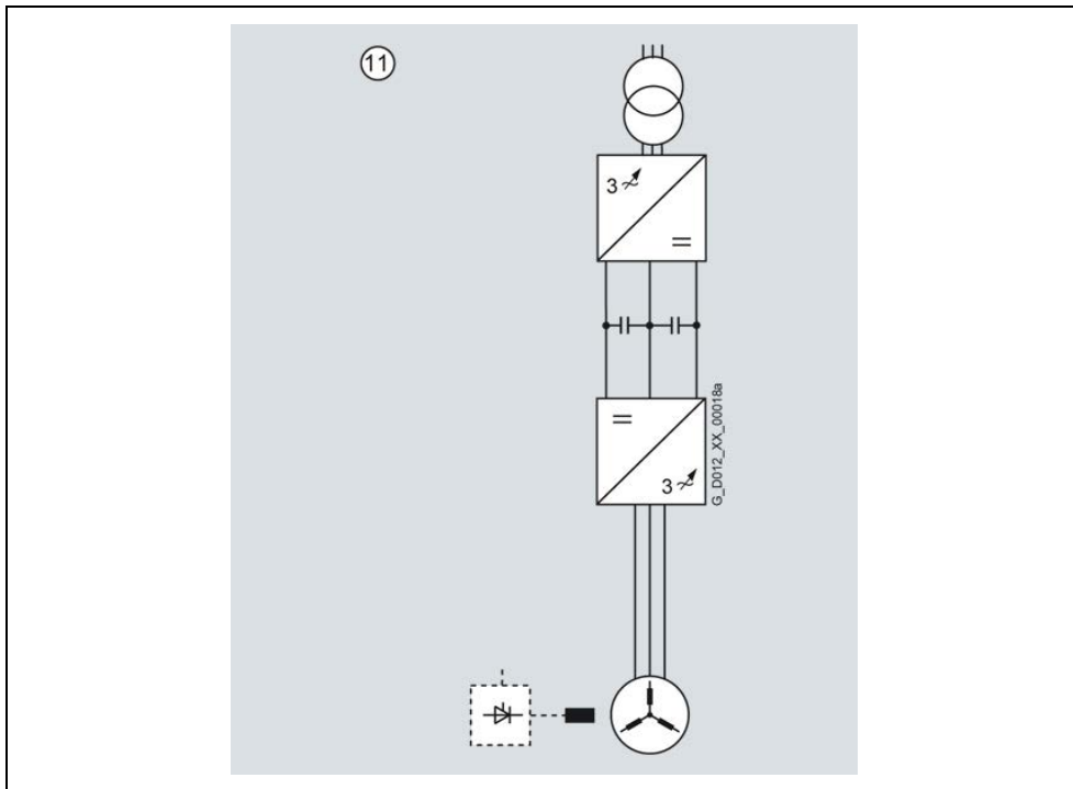
Fig. 5-4 Basic circuit
