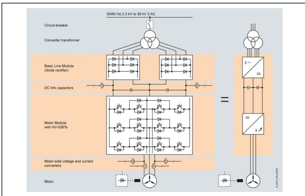
Fig. 2-3 Block diagram
