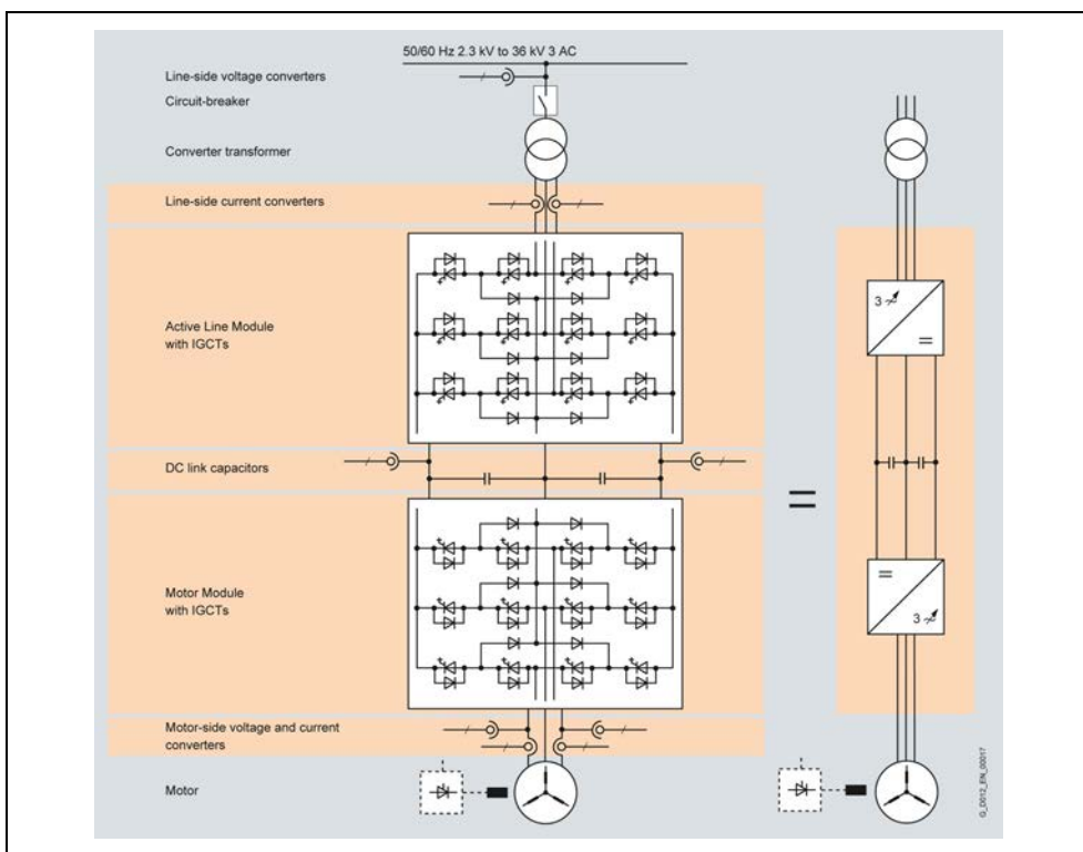
Fig. 5-3 Block diagram
