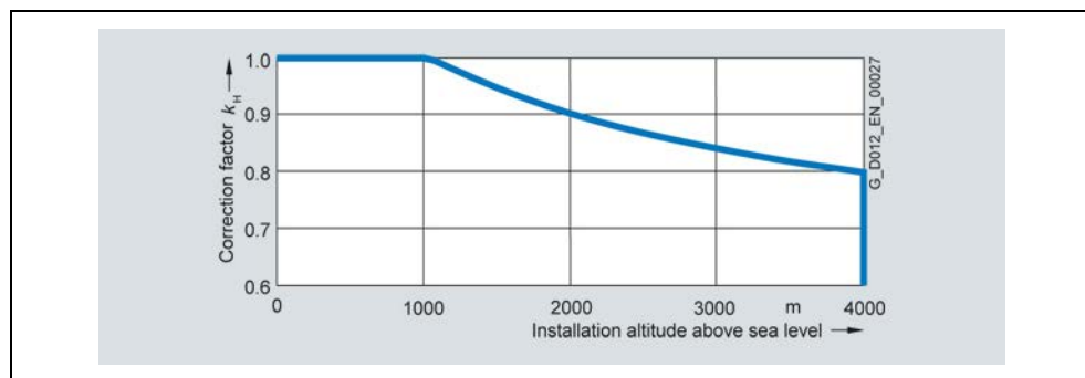
Fig. 2-9 Derating factor k_H for air cooling
