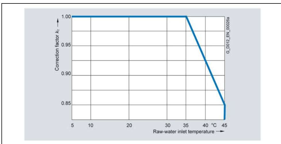
Fig. 4-8 Derating factor k_T (raw water intake temperature)
