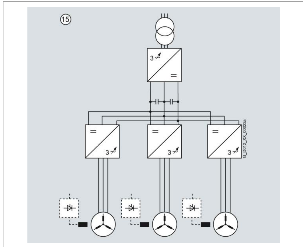
Fig. 5-8 DC bus configuration with three motors connected to a common DC link
