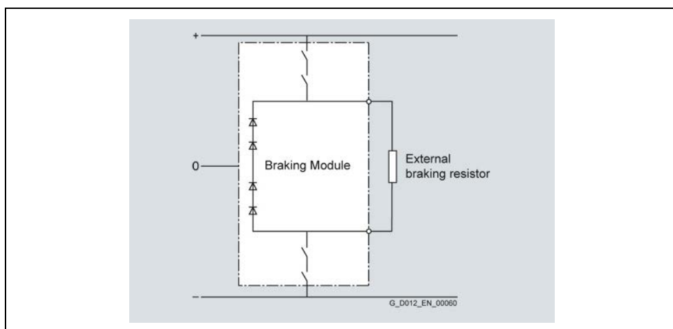
Fig. 7-5 Block diagram, Braking Module with braking resistor
