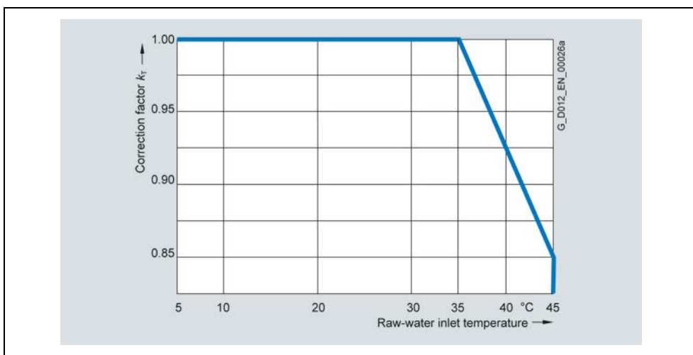
Fig. 2-12 Derating factor k_T (raw water intake temperature)
